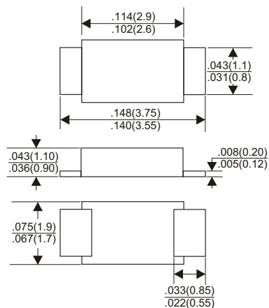
SOD123FL
